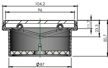
SECTION C-C SCALE 1 : 2
