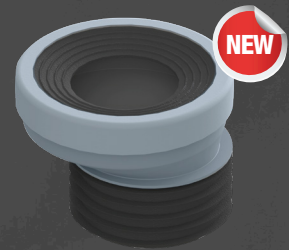
31906 100mm Pan Collar 20mm Offset w/ Flexi Fin Connection
