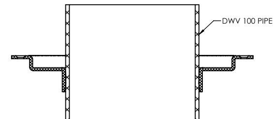
SECTION C-C
